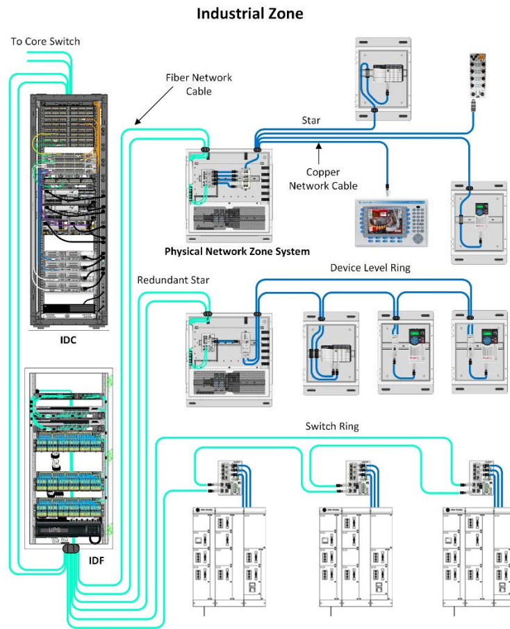
Figure 3. Physical Layout of Block Diagram.
