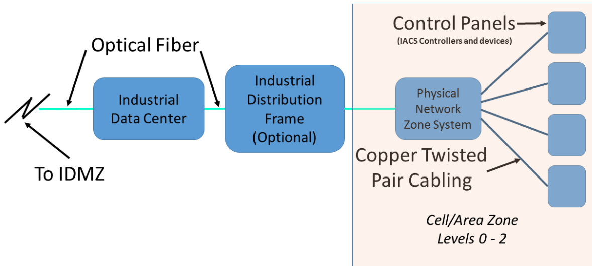
Figure 2. Logical Building Blocks Diagram.
