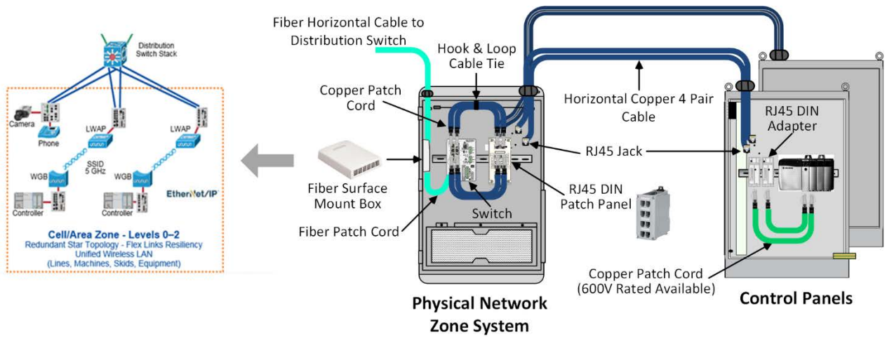
Figure 5. Example Redundant Star Topology.
