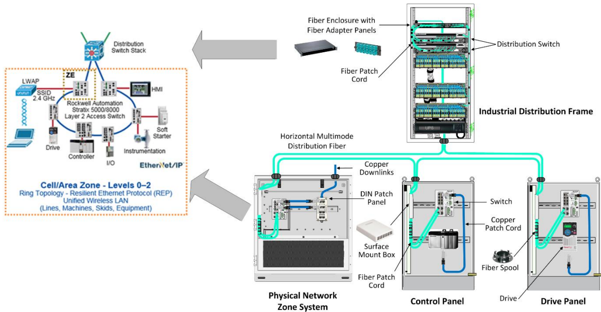
Figure 4. Example Switch-level Ring Topology.
