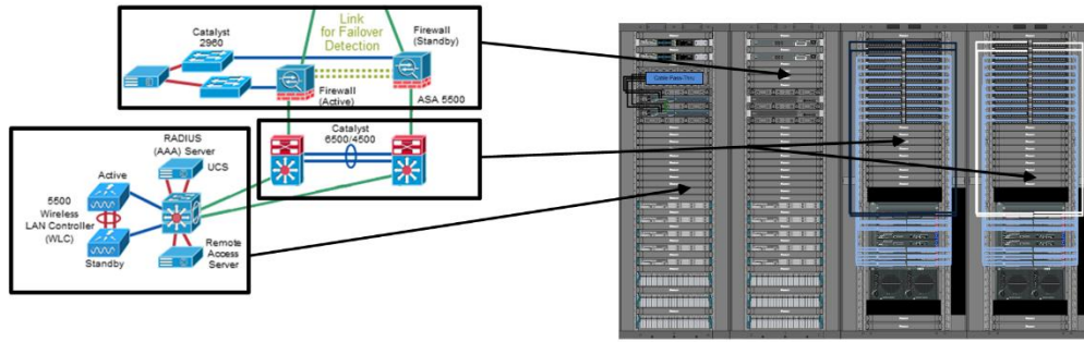
Figure 6. Level 3 Site Operations Layout.
