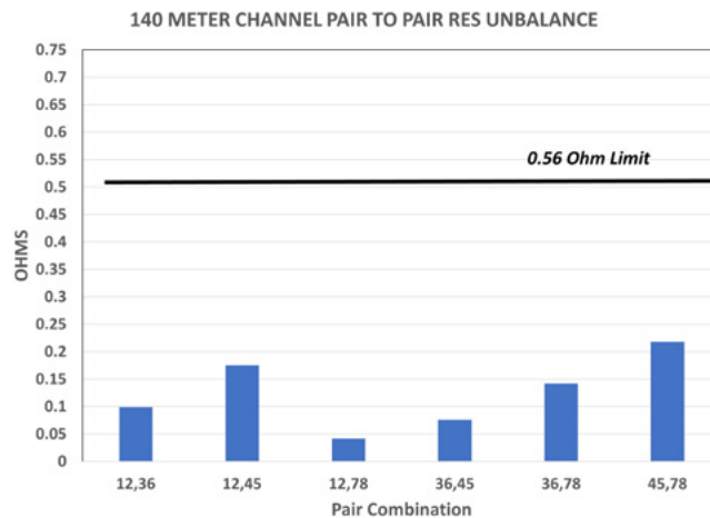
Figure 16: 140-meter channel pair-to-pair resistance unbalance (130-meter 22 AWG Category 6 cable, plus 10 meters of 24 AWG Category 6 patch cords)
