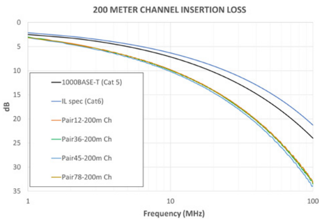
Figure 17: 200-meter channel insertion loss (190-meter 22 AWG Category 6 cable, plus 10 meters of 24 AWG Category 6 patch cords)
