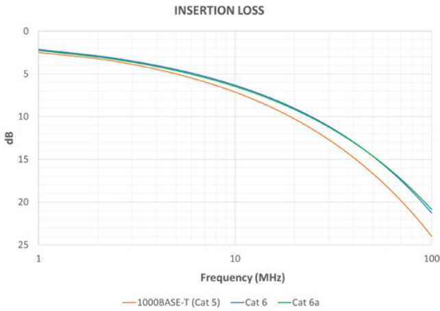
Figure 2: Insertion loss comparison between the 1000BASE-T specification and the Category 6 and 6A standards
