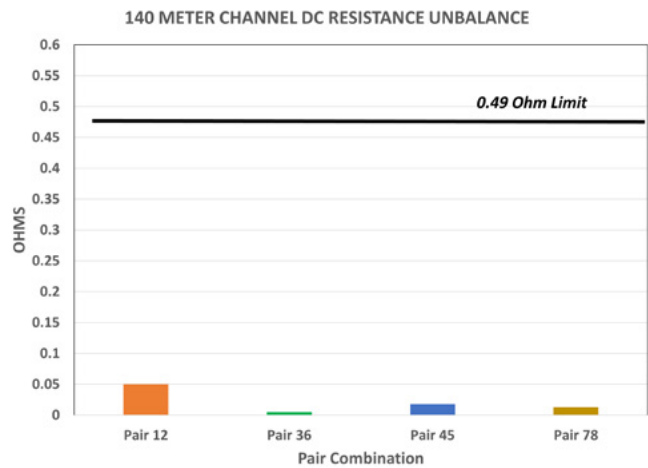
Figure 15: 140-meter channel resistance unbalance (130-meter 22 AWG Category 6 cable, plus 10 meters of 24 AWG Category 6 patch cords)
