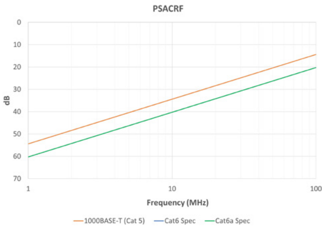
Figure 4: PSACRF comparison between the 1000BASE-T specification and the Category 6 and 6A standards
