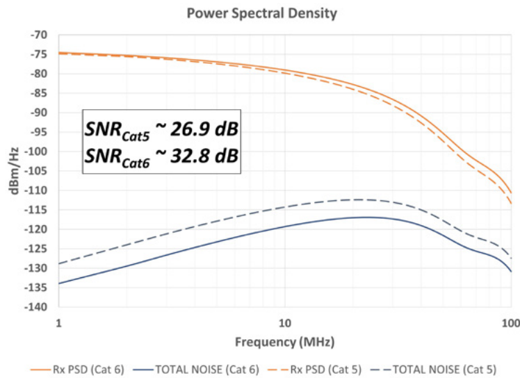
Figure 6: PSD of the noise for a Category 5 cabling channel, PSD of the noise for a Category 6 cabling channel, and the resulting PSD of the received 1000BASE-T signal transmitted over a Category 5 and Category 6 or 6A cabling system.
