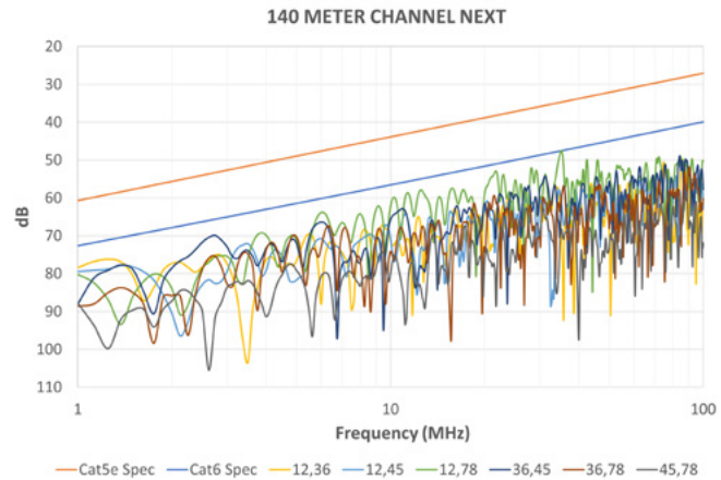
Figure 10: 140-meter channel NEXT (130-meter 22 AWG Category 6 cable, plus 10 meters of 24 AWG Category 6 patch cords)
