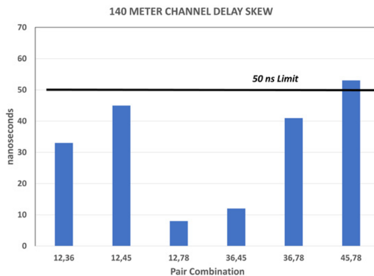
Figure 13: 140-meter channel Delay Skew (130-meter 22 AWG Category 6 cable, plus 10 meters of 24 AWG Category 6 patch cords)
