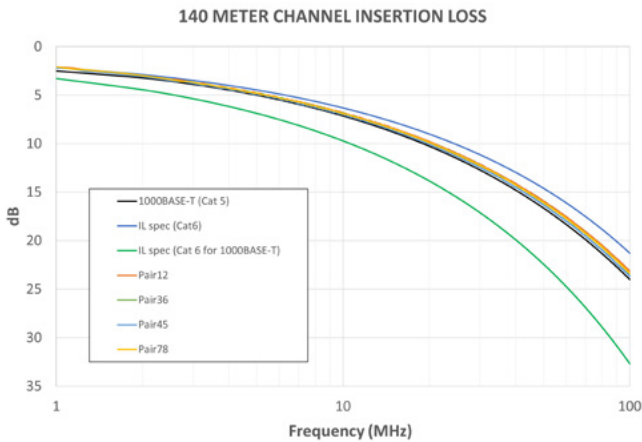
Figure 9: 140-meter channel insertion loss (130-meter 22 AWG Category 6 cable, plus 10 meters of 24 AWG Category 6 patch cords)
