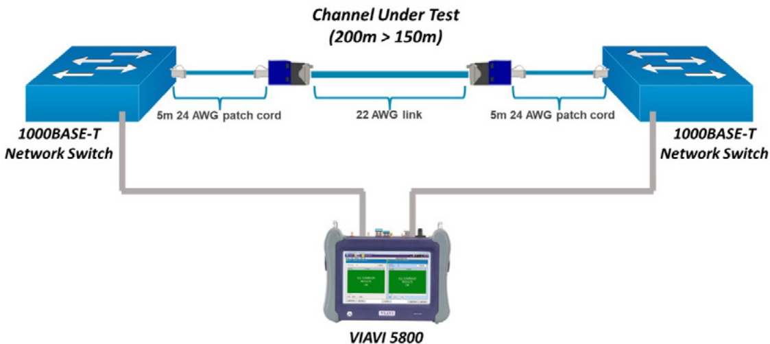
Figure 8: Test Channel Configuration
