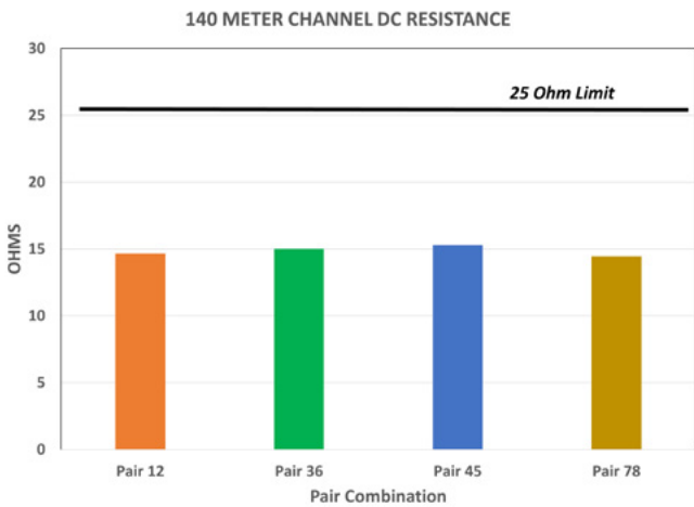
Figure 14: 140-meter channel DC resistance (130-meter 22 AWG Category 6 cable, plus 10 meters of 24 AWG Category 6 patch cords)
