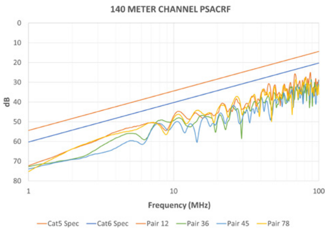
Figure 11: 140-meter channel PSACRF (130-meter 22 AWG Category 6 cable, plus 10 meters of 24 AWG Category 6 patch cords)
