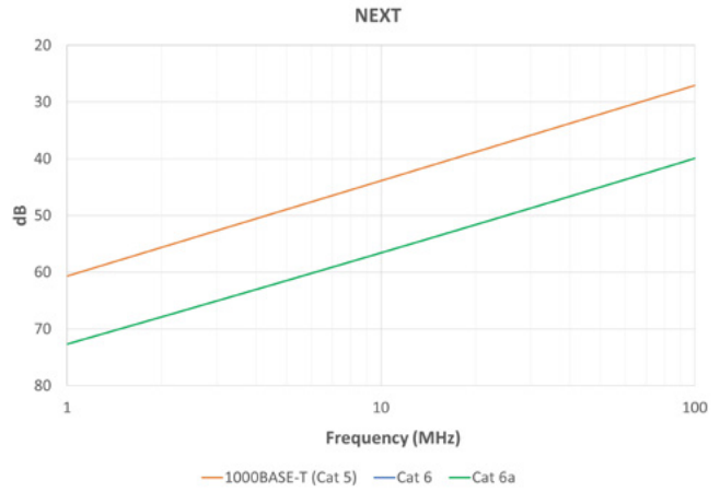
Figure 3: NEXT comparison between the 1000BASE-T specification and the Category 6 and 6A standards
