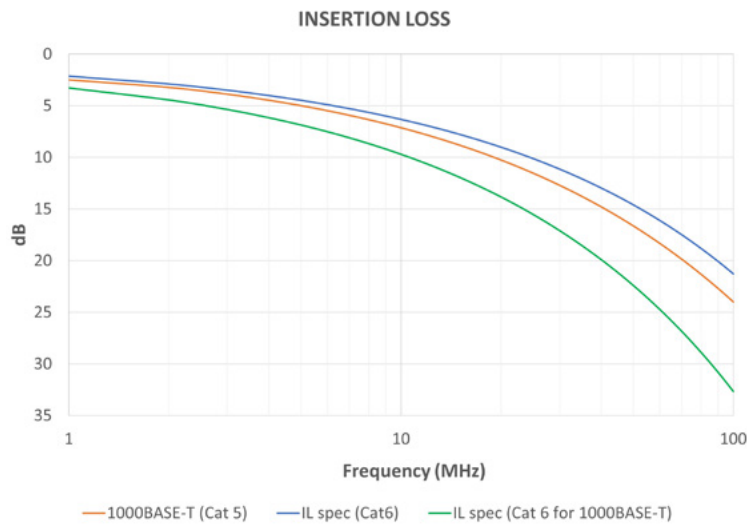
Figure 7: Theoretical maximum Category 6 insertion loss limit for 1000BASE-T links
