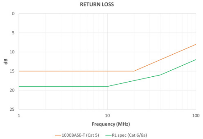
Figure 5: Return Loss comparison between the 1000BASE-T specification and the Category 6 and 6A standards
