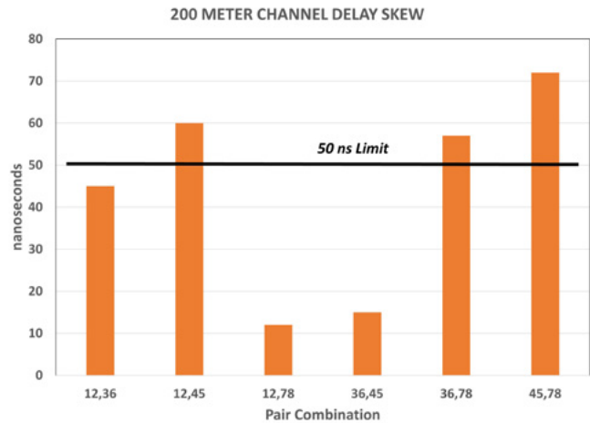
Figure 18: 200-meter channel delay skew (190-meter 22 AWG Category 6 cable, plus 10 meters of 24 AWG Category 6 patch cords)
