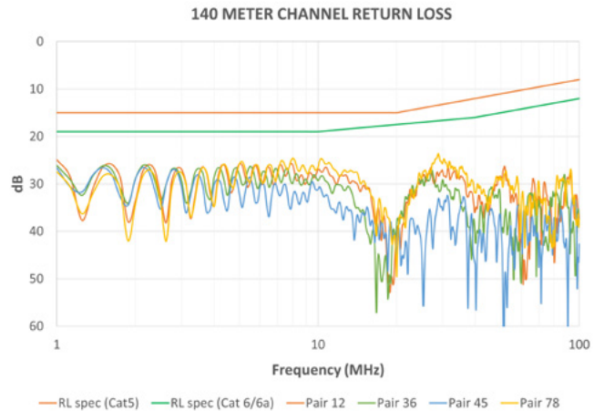
Figure 12: 140-meter channel Return Loss (130-meter 22 AWG Category 6 cable, plus 10 meters of 24 AWG Category 6 patch cords)
