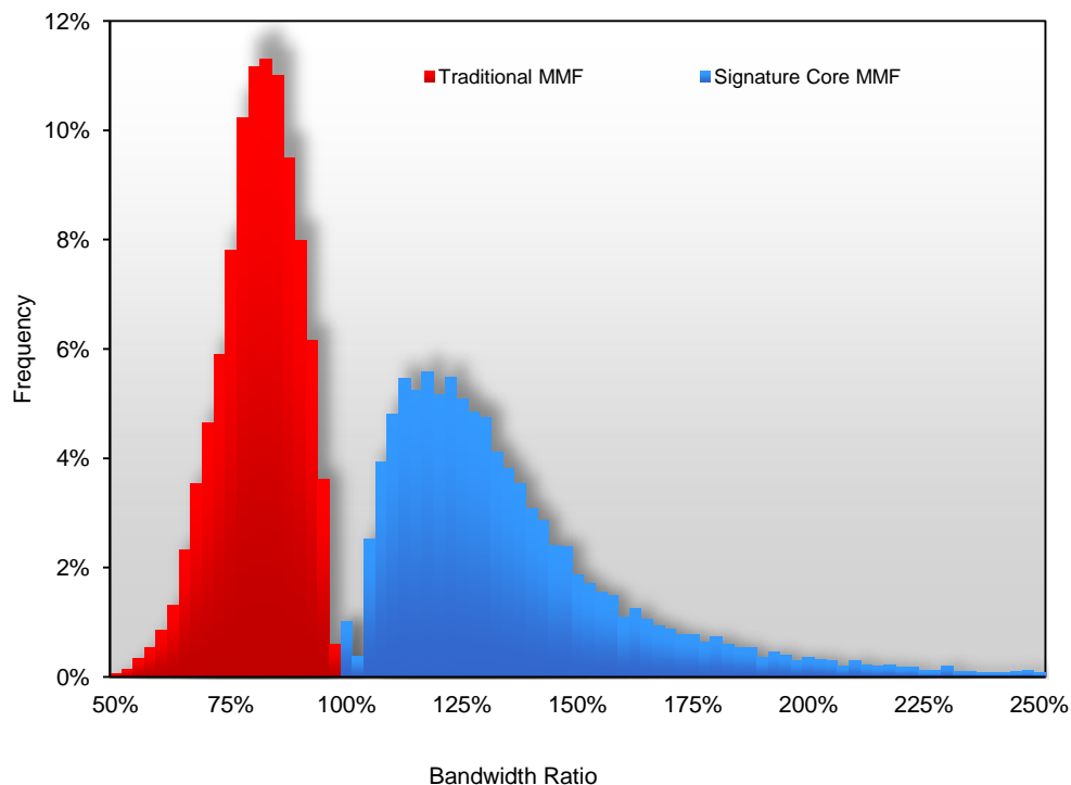
Figure 4. Modeled benefit, in terms of bandwidth ratio of Panduit's Signature Core™ Fiber Optic Cabling System compared to traditional MMF that does not compensate modal and chromatic dispersion.
