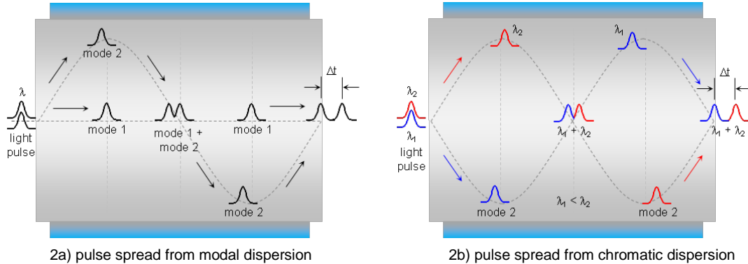
Figure 2. Simplified representation of 2a) modal dispersion and 2b) chromatic dispersion in MMF.
