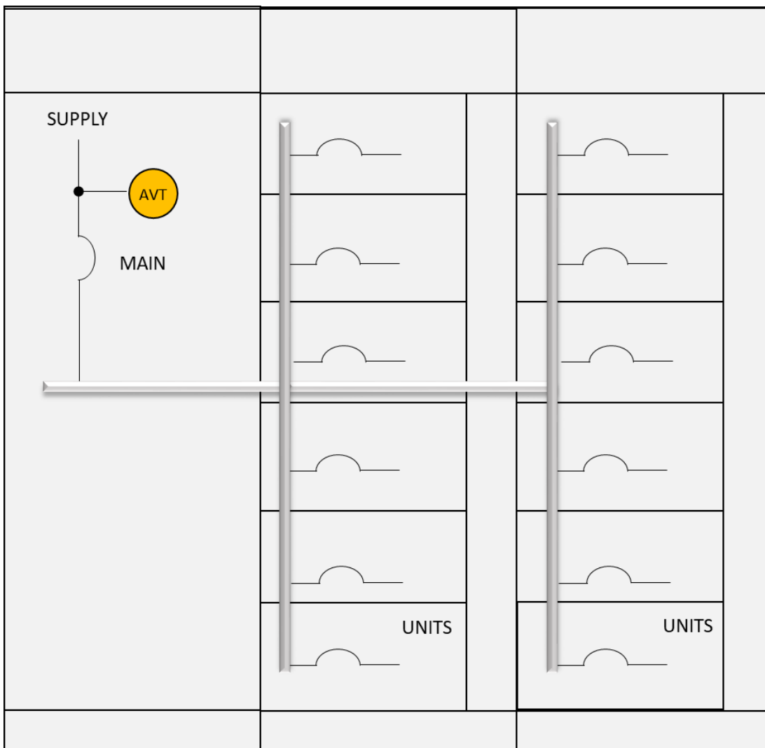
Figure 2: AVT Installed on Line Side of Main
