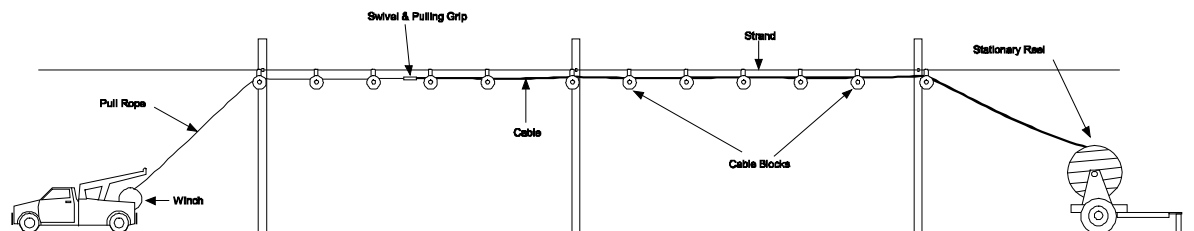
Figure 2. - The stationary reel method of cable placement
