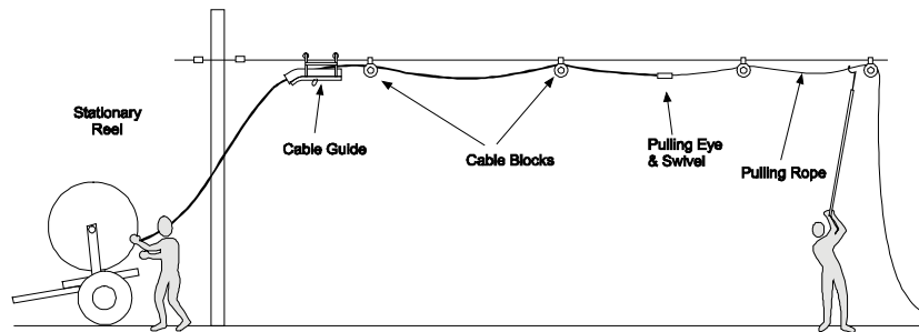
Figure 8 - Setup for stationary reel method
