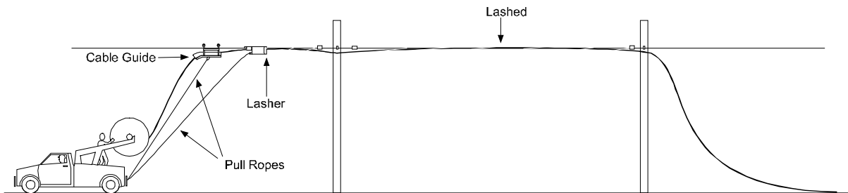
Figure 1. - The moving reel method of cable placement
