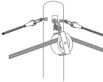
Figure 9 - Snatch block
