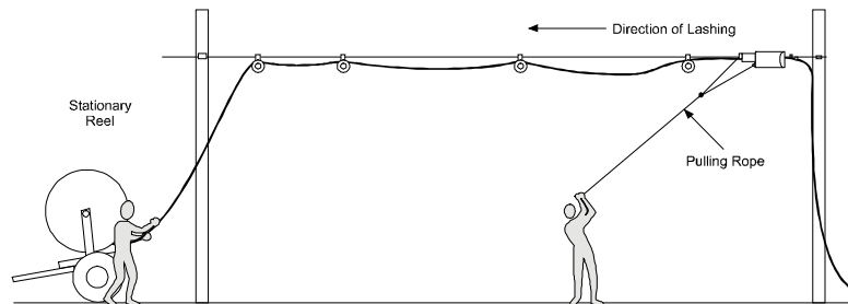
Figure 10 - Pull-back lashing of cable
