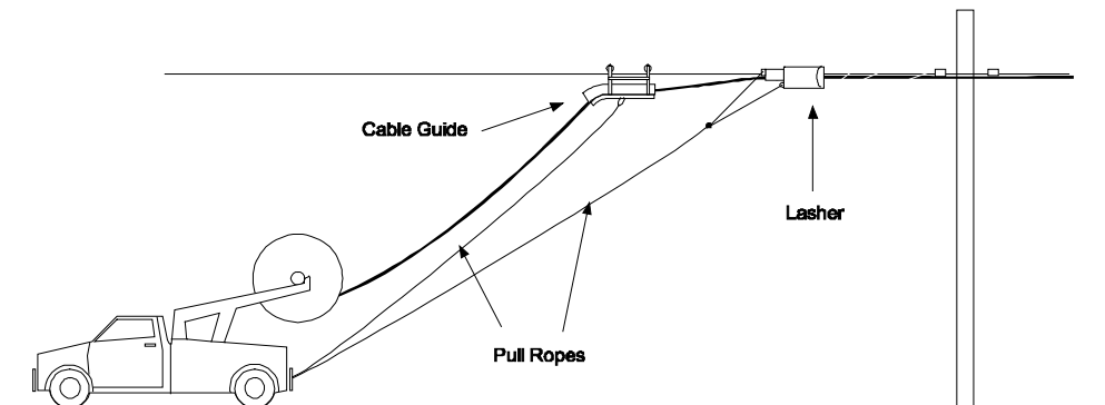
Figure 7 - Setup for moving reel method
