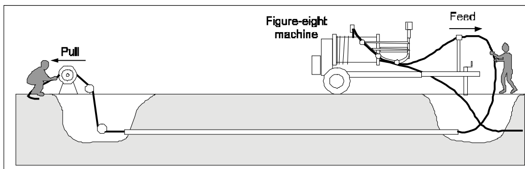
Figure 6 – Pulling Using a Figure-eight Machine
