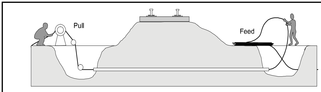
Figure 4 – Pulling the Cable
