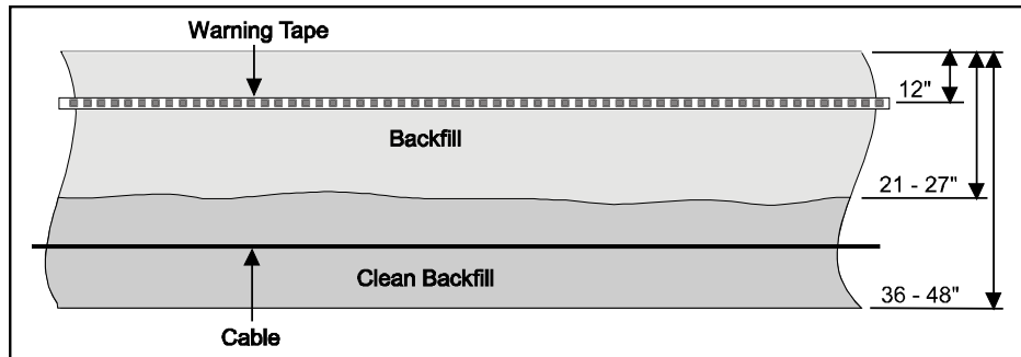
Figure 7 –Cutaway View of Buried Cable
