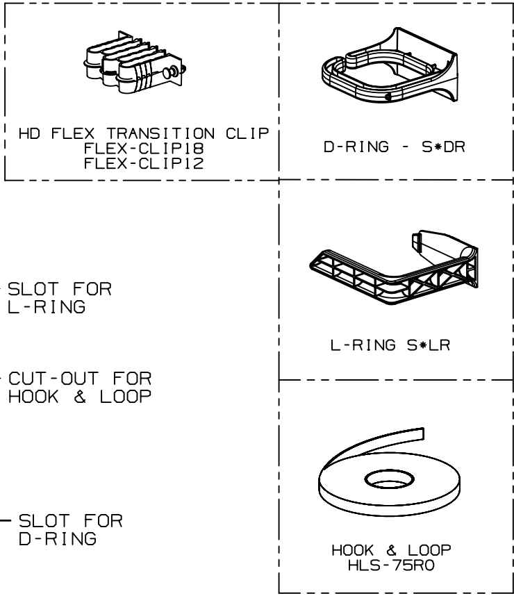
DETAIL A OPTIONAL-NOT INCLUDED VERTICAL CABLE MANAGER PANEL OPTIONS
