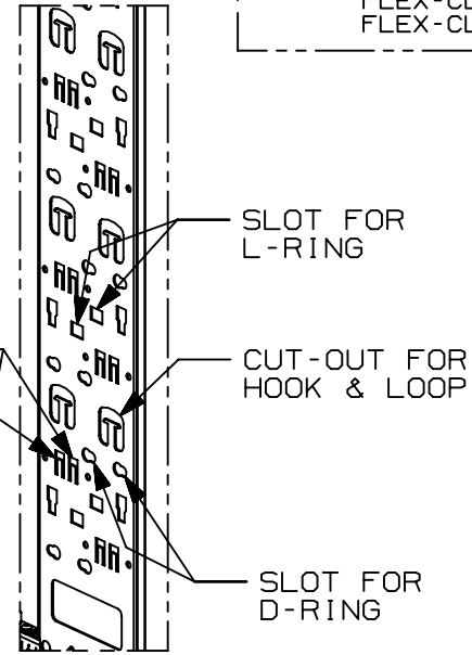
DETAIL A OPTIONAL-NOT INCLUDED VERTICAL CABLE MANAGER PANEL OPTIONS
