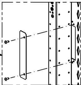
VIEW BN 600mm E-RAIL ARRANGEMENT NO PASS THRU OPENINGS
