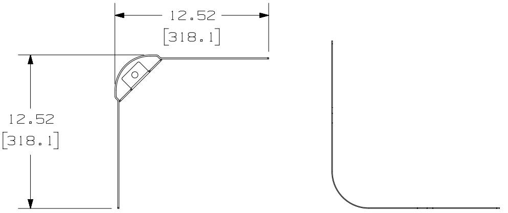
SUPPORT BRACKET BEND RADIUS PROTECTOR
