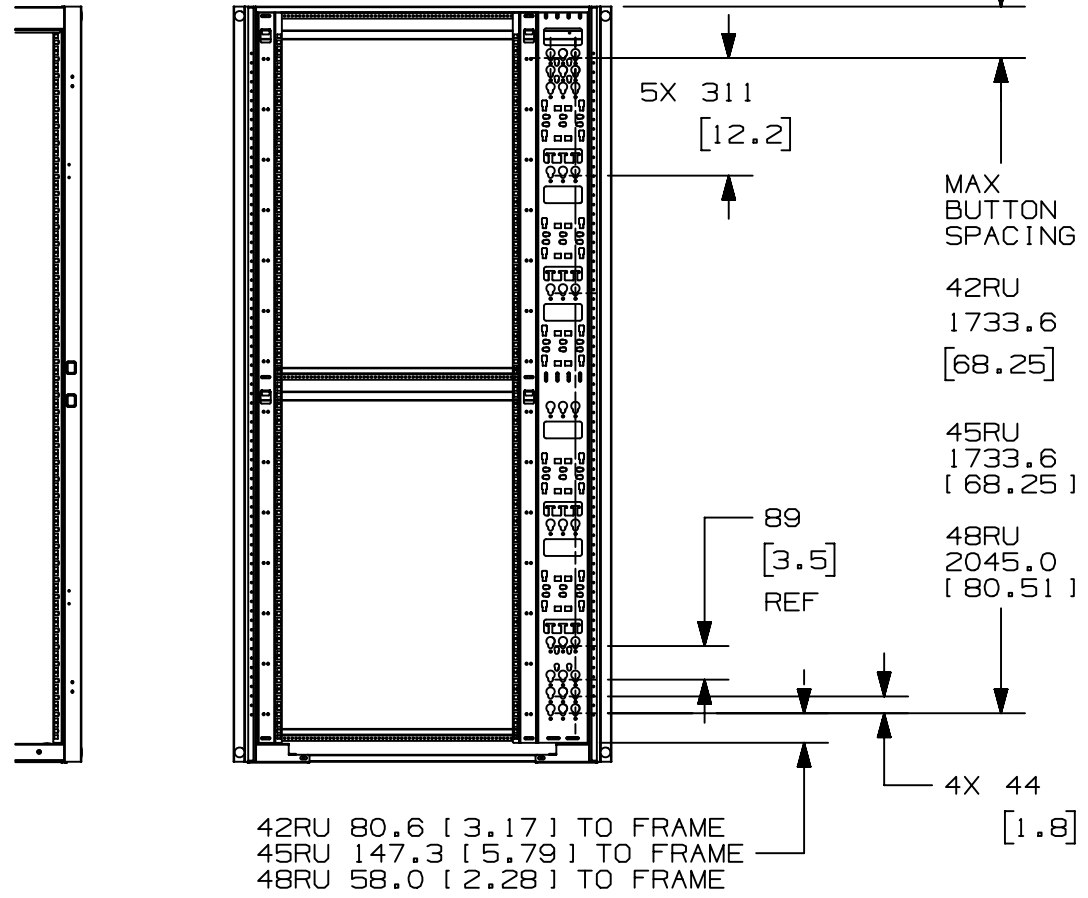
REAR VIEW
