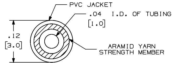
CROSS SECTION OF FURCATION TUBING
