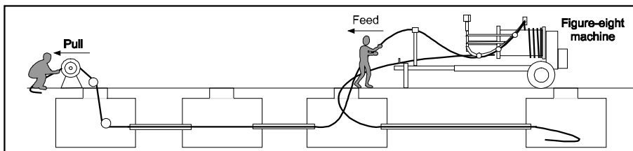
Figure 9 - Pulling using a figure-eight machine
