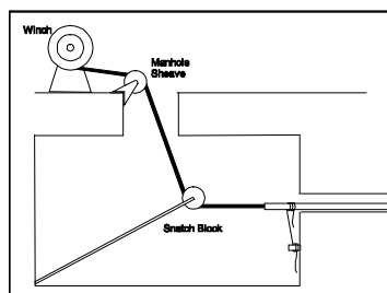
Figure 3 - Pull manhole setup
