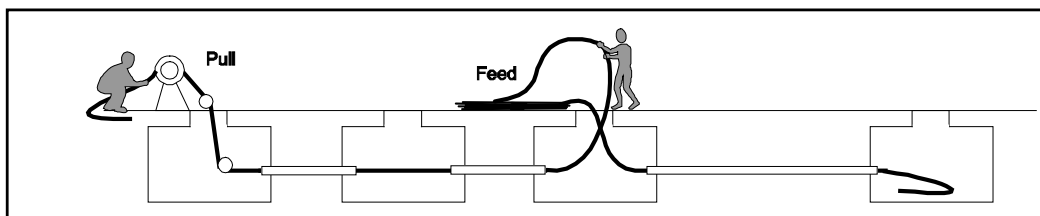
Figure 7 - Bi-directional pull completion
