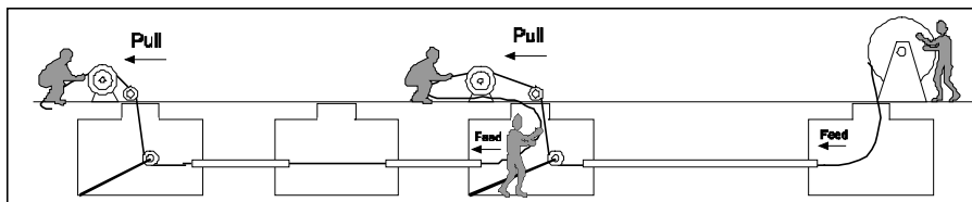
Figure 10 - Mid-pull assist setup
