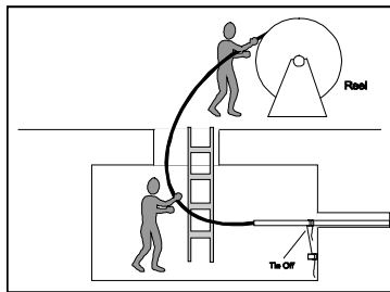
Figure 4 - Reel end setup
