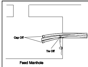
Figure 2 - Cable tie-off in manhole
