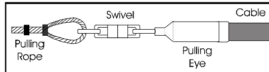
Figure 1 - 600# Break-away swivel and pulling eye
