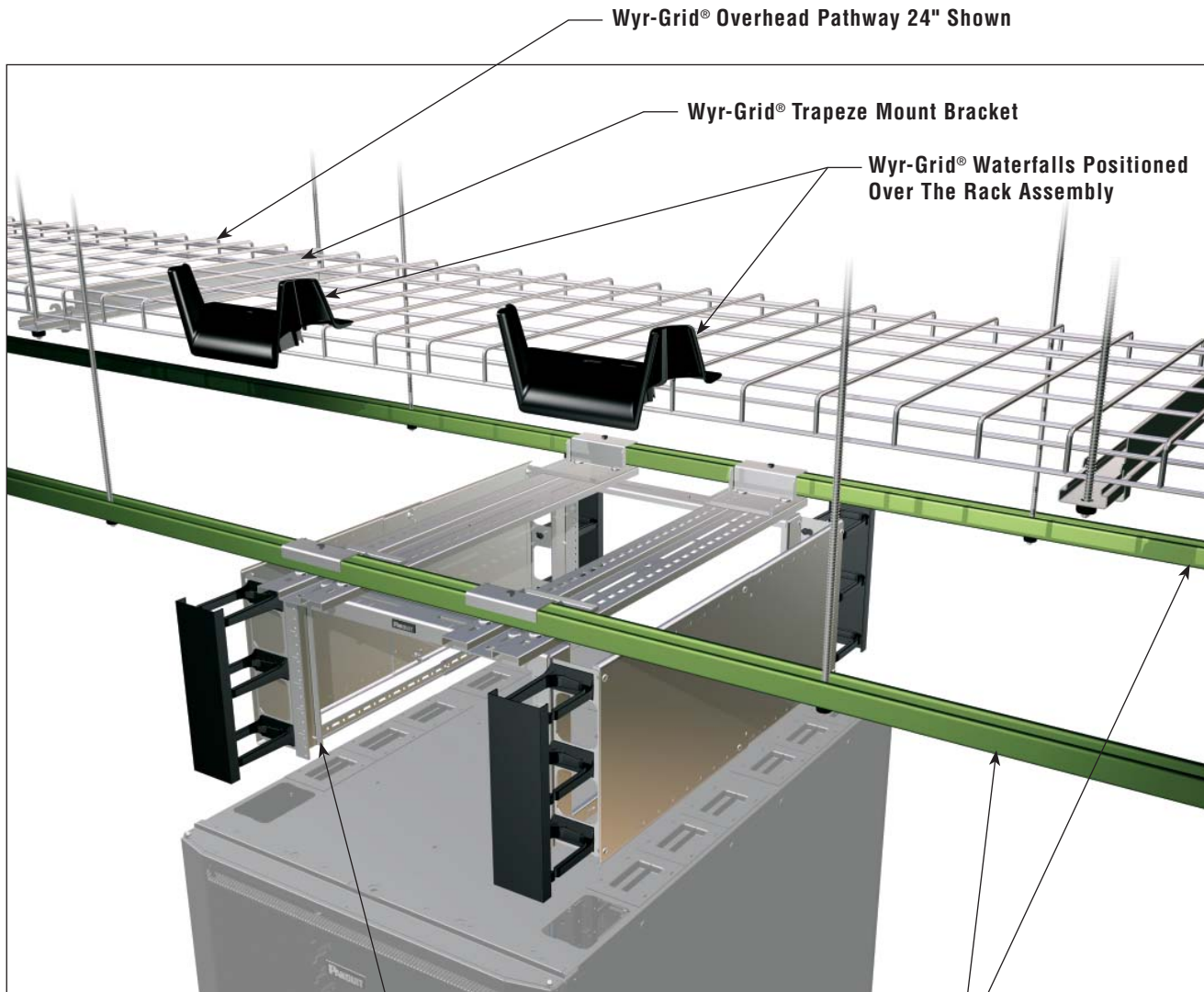
Assembled Overhead Rack Mounted to the Overhead Grid Strut Channels
