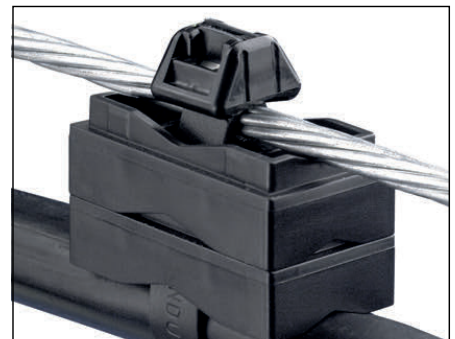
Stackable Aerial Cable Spacer Designed for use in parallel or perpendicular applications with Dura-Ty™ Cable Ties
