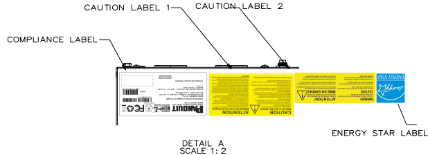
DETAIL A SCALE 1:2
