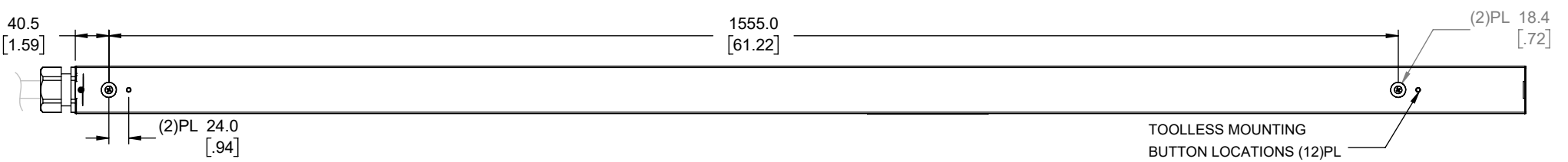
REAR VIEW
