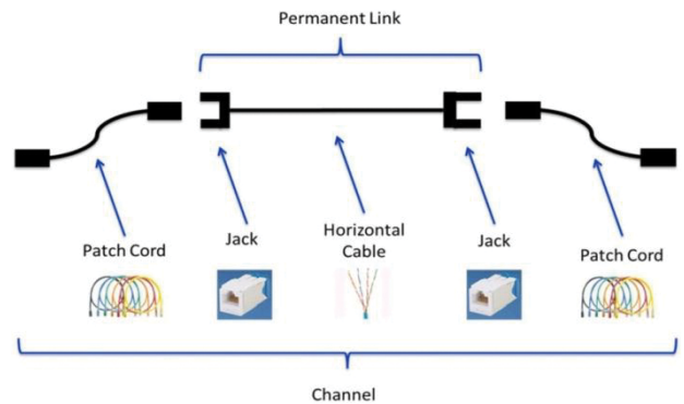
Figure 3. Simplified Example of Copper Structured Cabling.
