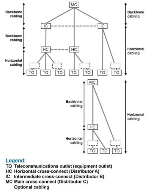
Figure 2. Elements of a Generic Cabling Topology.
