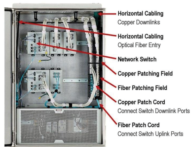
Figure 4. Integrated Network Zone System permanent link implementation.
