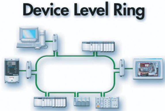
Figure 6. The Use of Point to Point Cabling in a Device Level Ring Topology. (Rockwell Automation).
