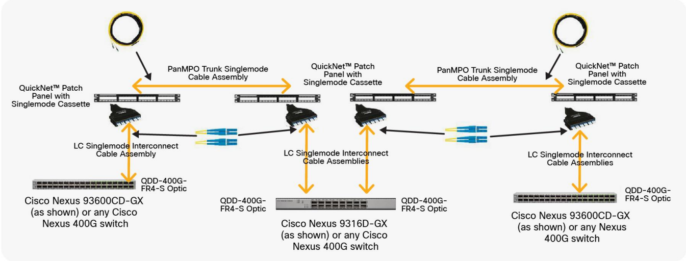
Figure 6. Cisco Nexus 9316D-GX to Cisco Nexus 93600CD-GX LC duplex to LC duplex single-mode cabling components
