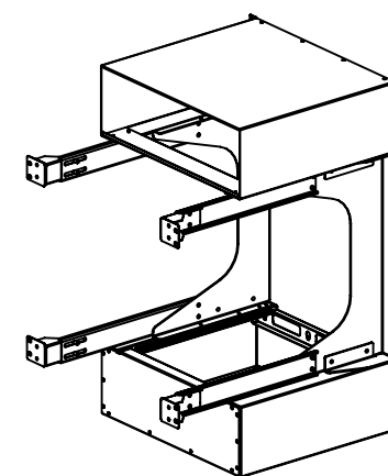
ISO VIEW
