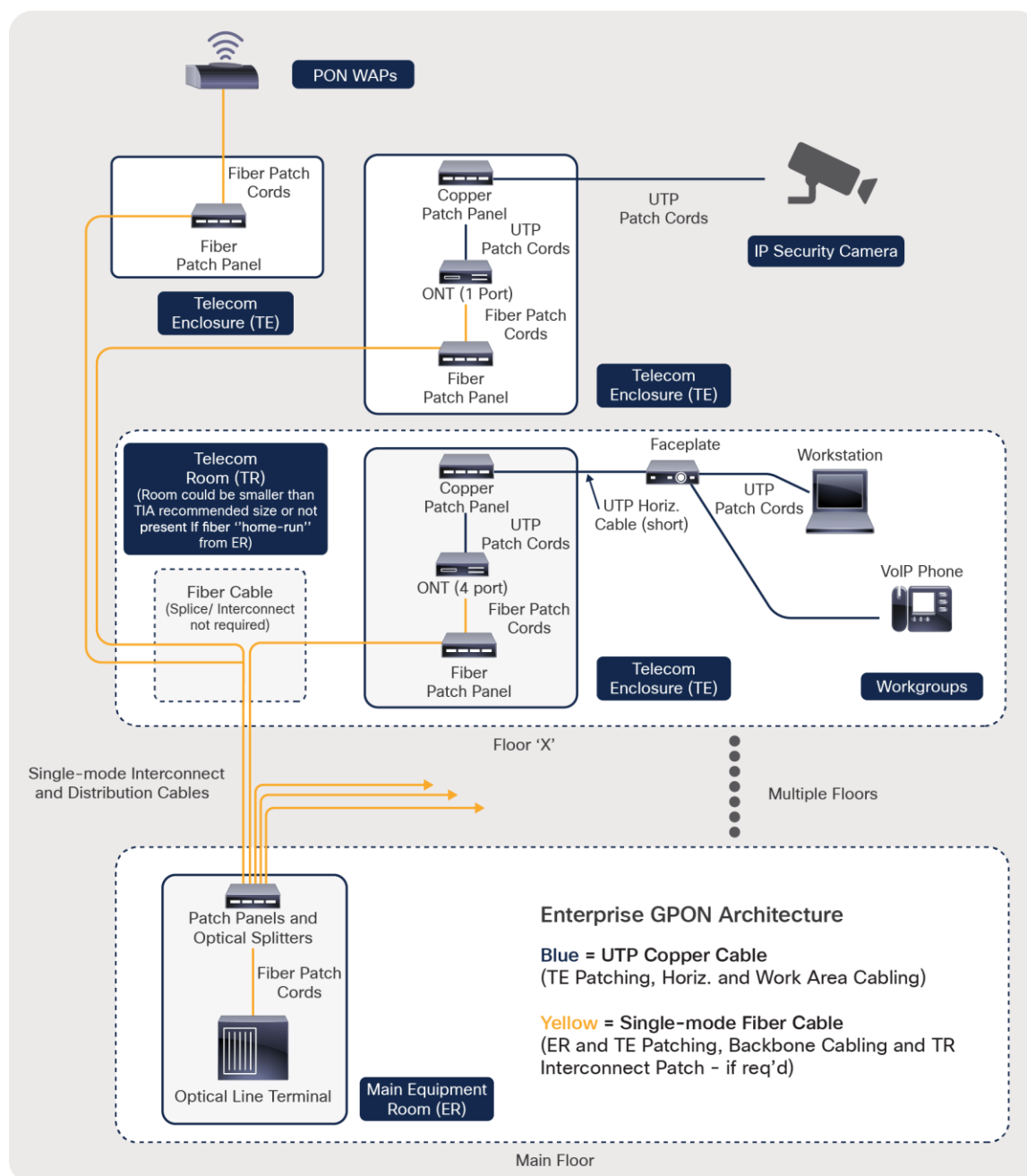
Figure 4. Deployment of zone-based ONTs via telecom enclosures
