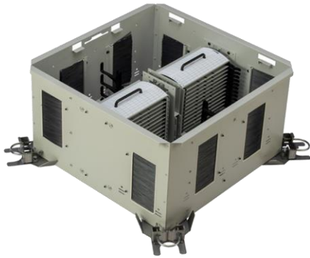
Figure 6. Raised floor enclosure (zone application)
