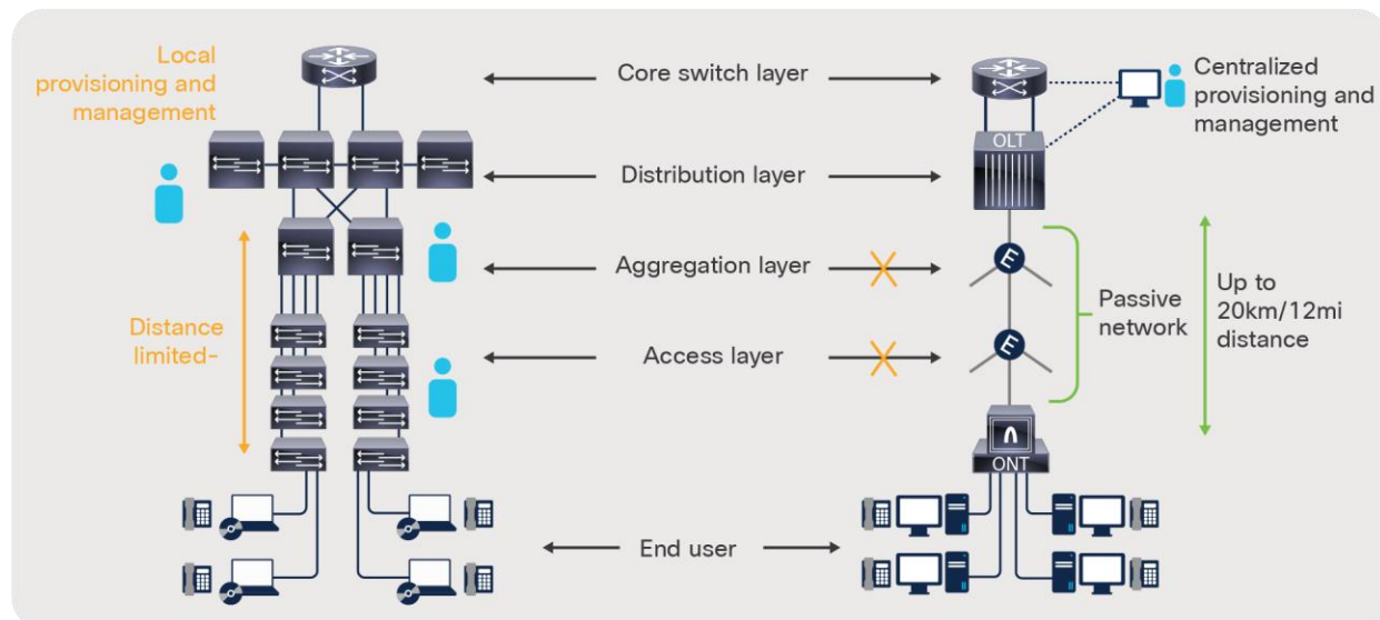
Figure 1. Active Ethernet network vs. passive optical LAN network
