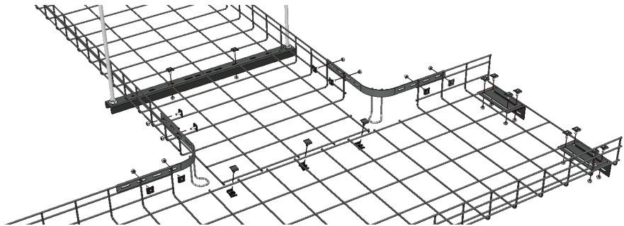
PWBSPL** -L Bolted Style Splice (Std. Pkg Qty = 50)
