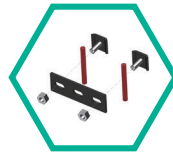
3-Hole Sweeping Bend Splice Bar Fabricated From PWBSPL5**-L with PWBHK**-L Hardware Kits
