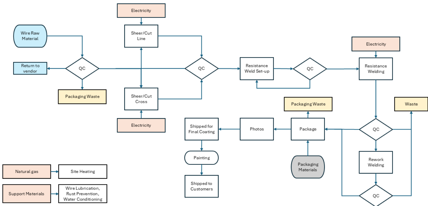
Wire Basket Manufacturing Process Flow Diagram
