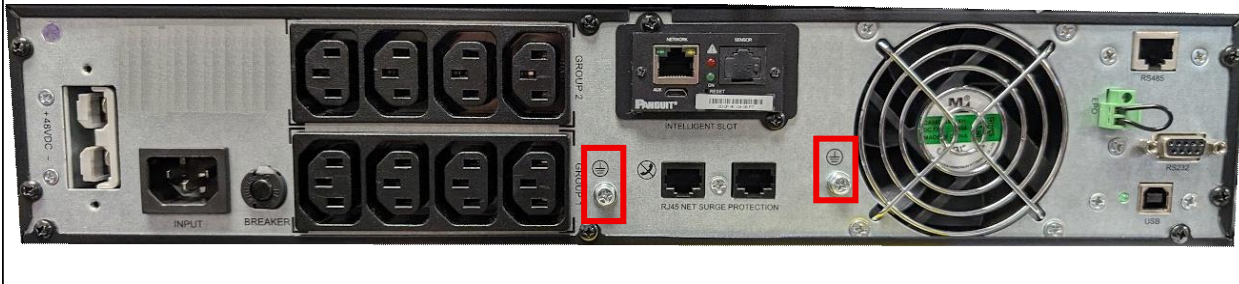
Grounding Locations (U01N18L-N Example)
