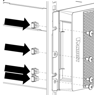
Figure 44: Install Cage Nuts in the Front Equipment Rail with Square Holes
