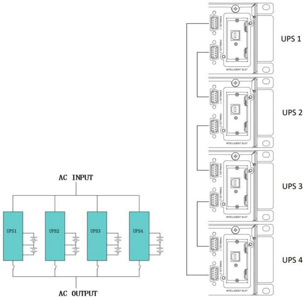
Figure 68a: Parallel System Power/Control Connections
