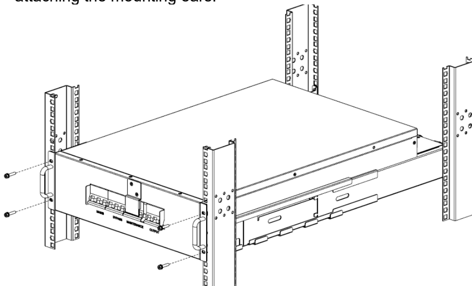
Figure 43: Secure the Mounting Brackets to the Rack
