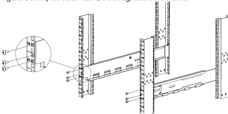
Figure 1: Install the Front Side of Rails
