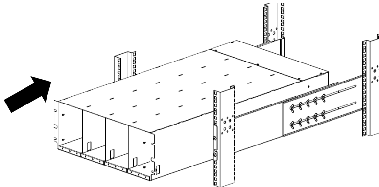
Figure 51: Slide EBP into Rack
