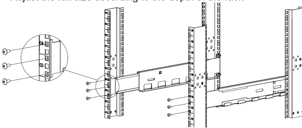
Figure 26: Install the Rear Side of Rails
