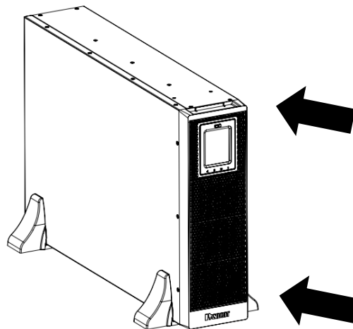
Figure 64: Example of Snapping the Faceplate onto the Front of the UPS
