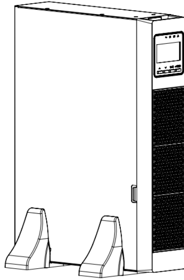
Figure 55b: 2U Unit using Tower Kit (Single Phase UPS example shown.)
