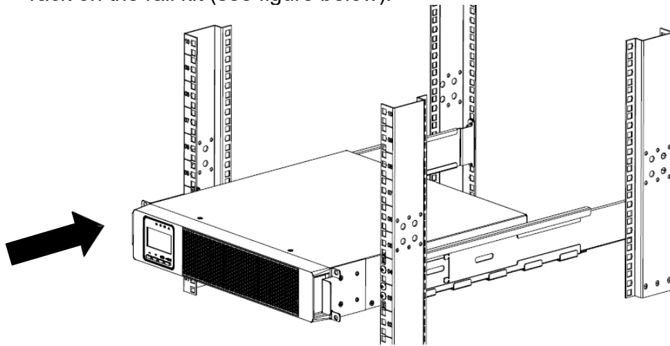
Figure 8: Slide the unit into the Rack (UPS example shown)
