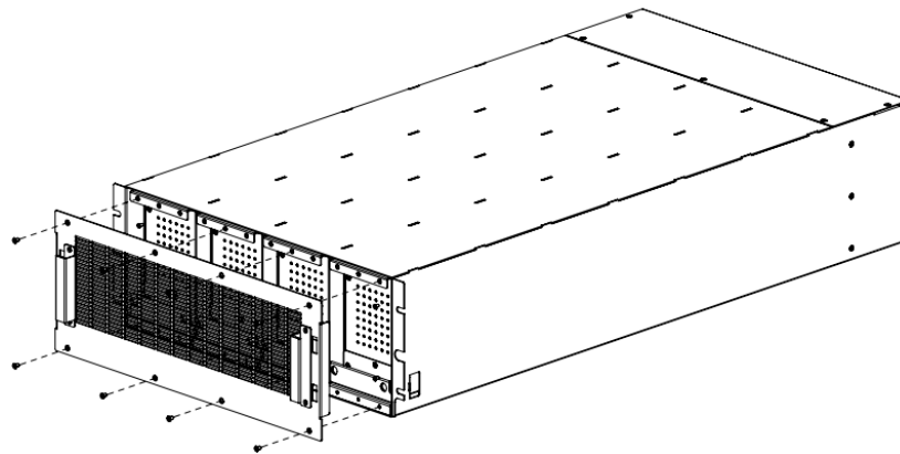
Figure 49: Remove Battery Baffle on the EBP
