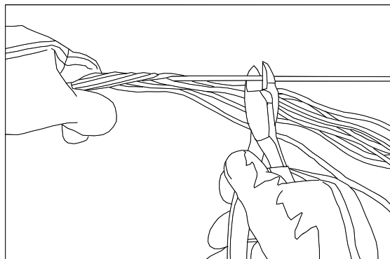
(Figure 3.2.c) Cut central member to proper length with cable cutters
