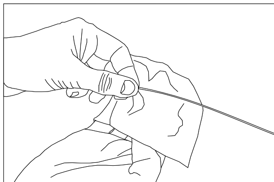
(Figure 3.3.b) Wipe excess thixotropic gel from the fibers or ribbons
