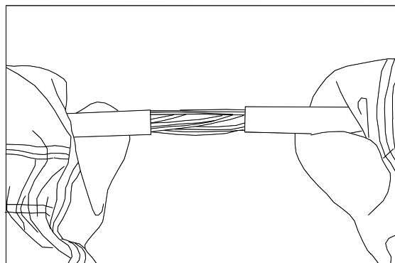
(Figure 3.1.b) Remove the cable end sheath section
