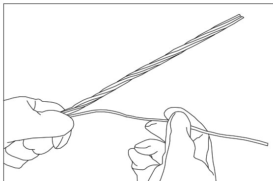
(Figure 3.2.b) Separate buffer tubes from central member.
