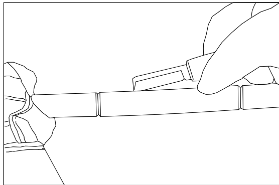
(Figure 4.2.e) Ring cuts 3 – 5 inches apart and flexed. Find armor overlap at ring cut, slit the sheath over top of the overlap and peel back
