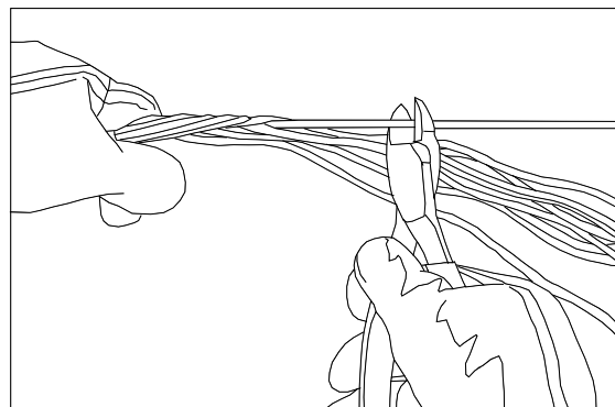
(Figure 4.3.b) Cutting the central strength member with cable cutters
