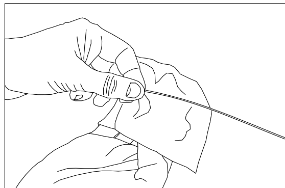
(Figure 4.4.d) Wipe excess thixotropic gel from the fibers or ribbons
