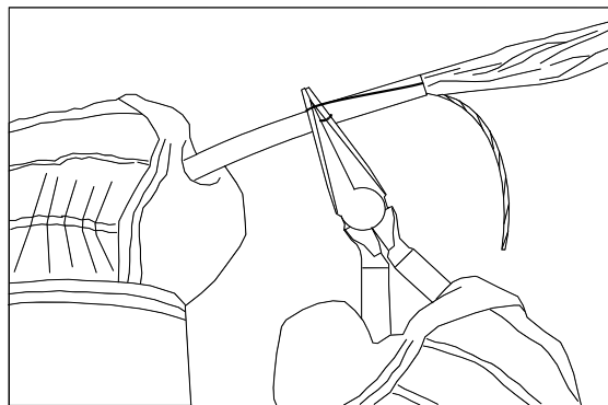
(Figure 3.1.c) Grasp and pull ripcord with needle nose pliers
