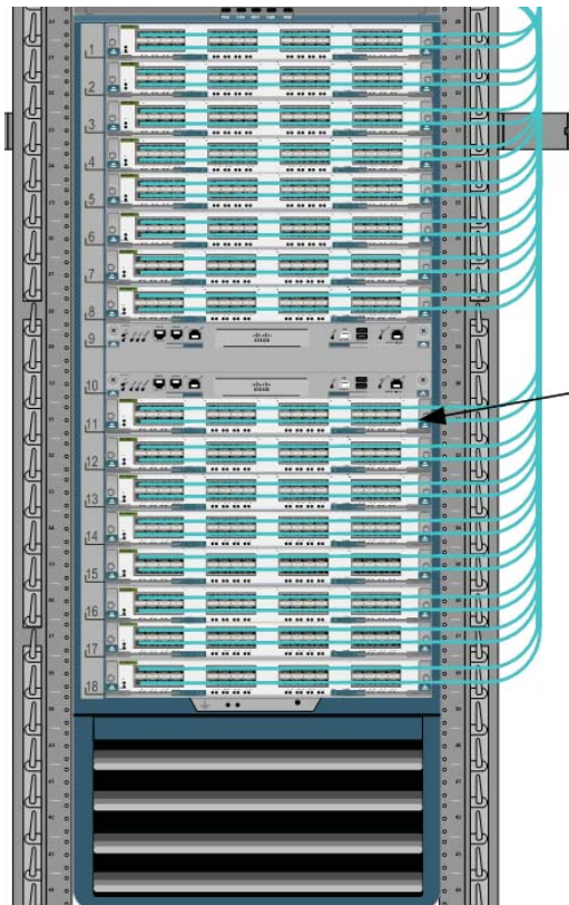
Hydra cable assemblies consolidate LC connectivity into one multi-array adapter (Example showing a Nexus 7018)
