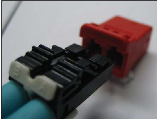
Figure 2. LCTRDC meets FOCIS-10a specifications
